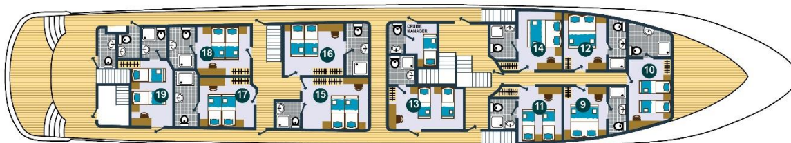
MAIN DECK
